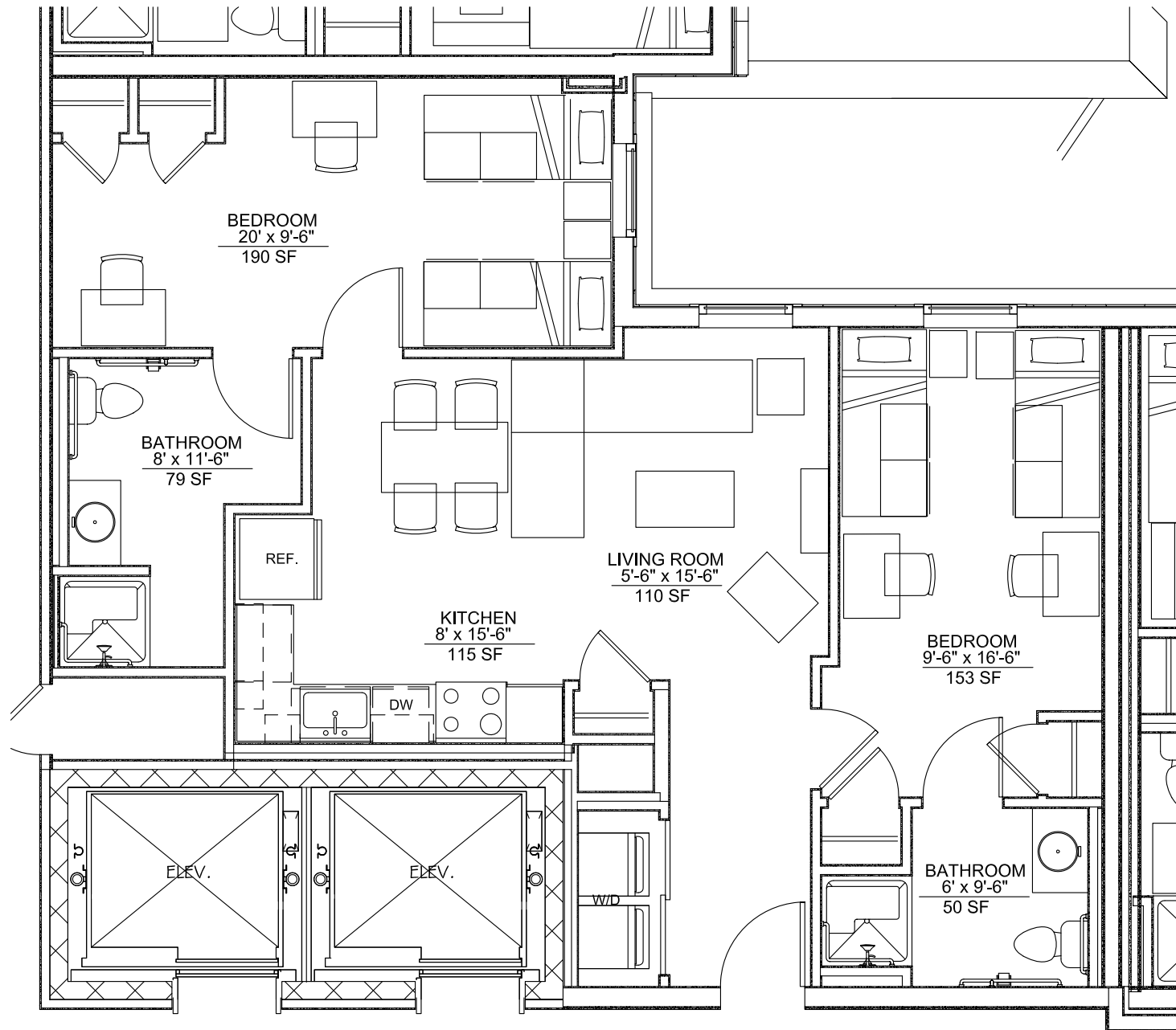
FURNITURE TYPICAL 9 TWO BEDROOM HC CORNER SUITE
