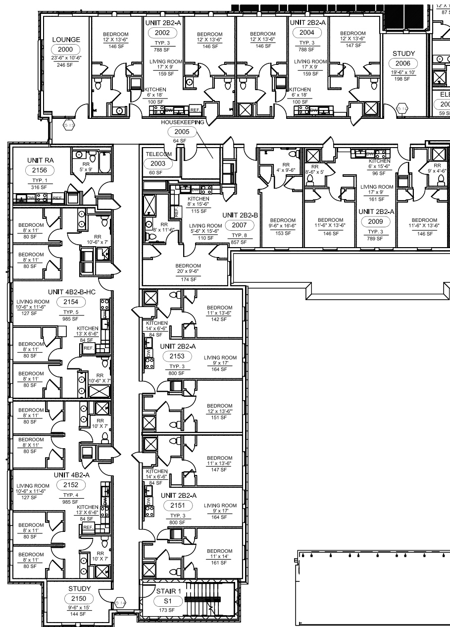
AREA A - SECOND FLOOR NOT TO SCALE
