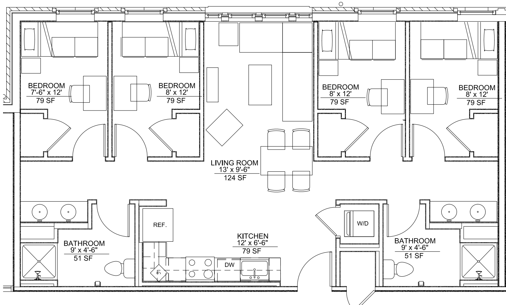
FURNITURE TYPICAL 4 FOUR BEDROOM UNIT
