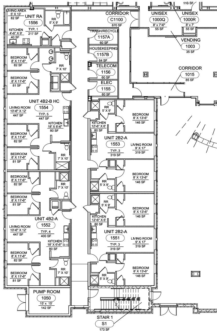
AREA A1 - FIRST FLOOR NOT TO SCALE
