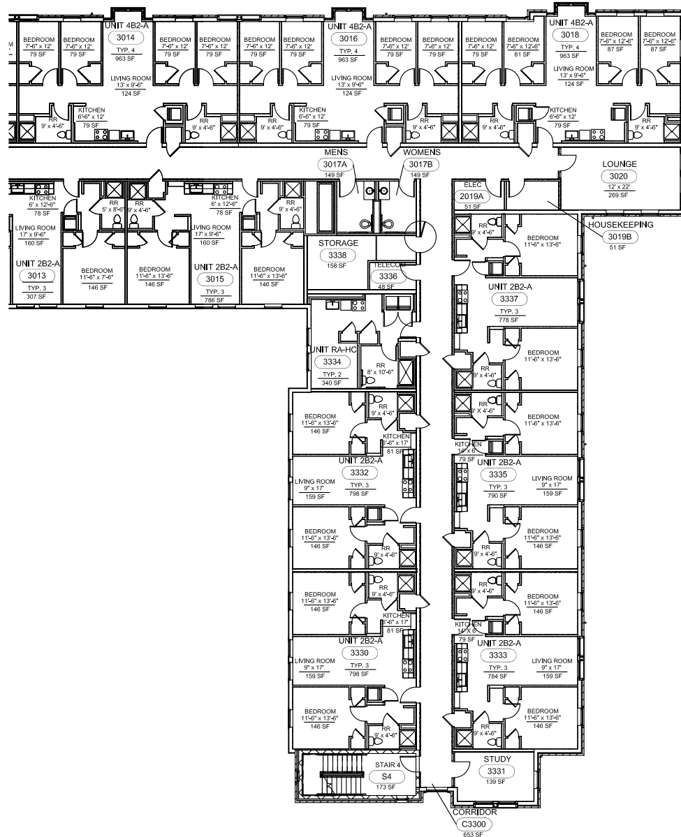
AREA C - THIRD FLOOR NOT TO SCALE
