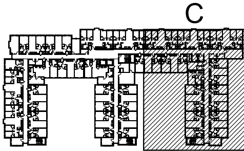
KEY PLAN THIRD FLOOR
