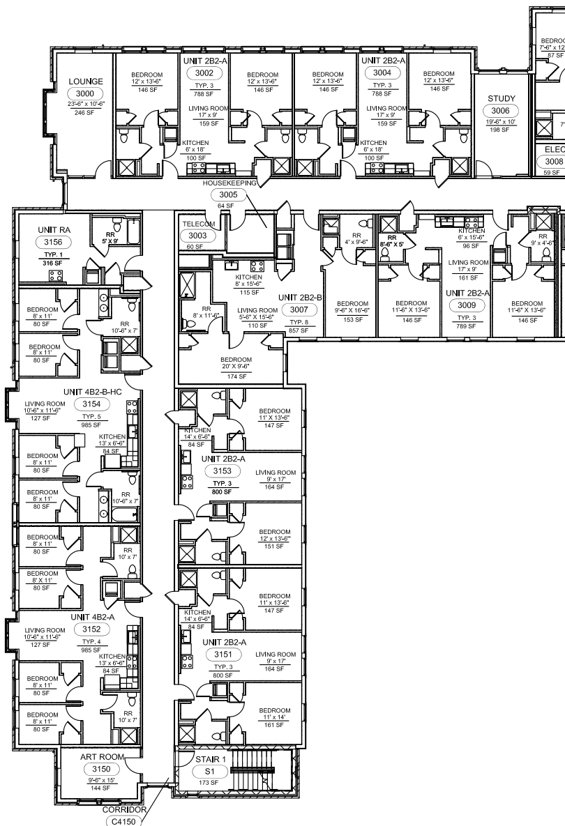
AREA A - THIRD FLOOR NOT TO SCALE
