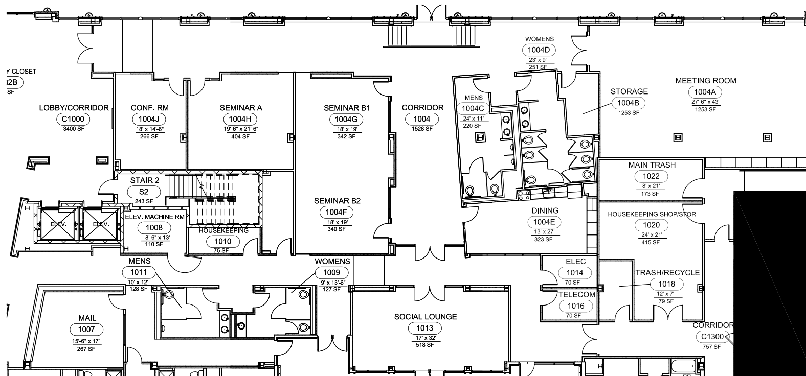
AREA D - FIRST FLOOR NOT TO SCALE
