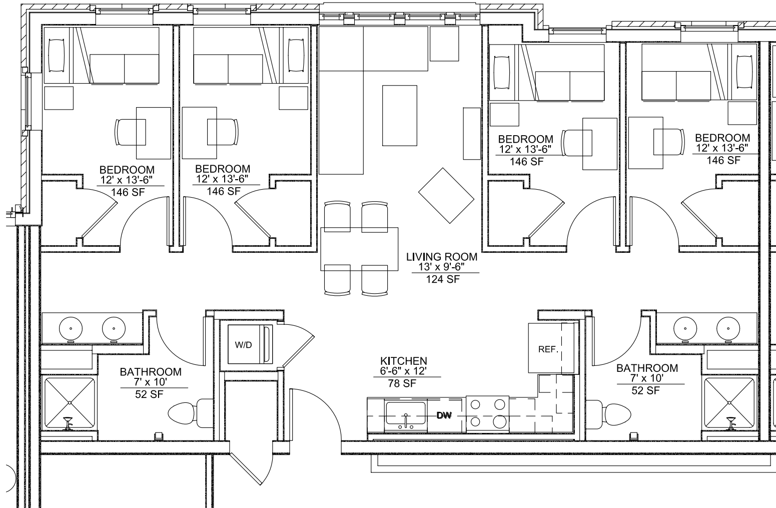
FURNITURE TYPICAL 6 FOUR BEDROOM SUITE
