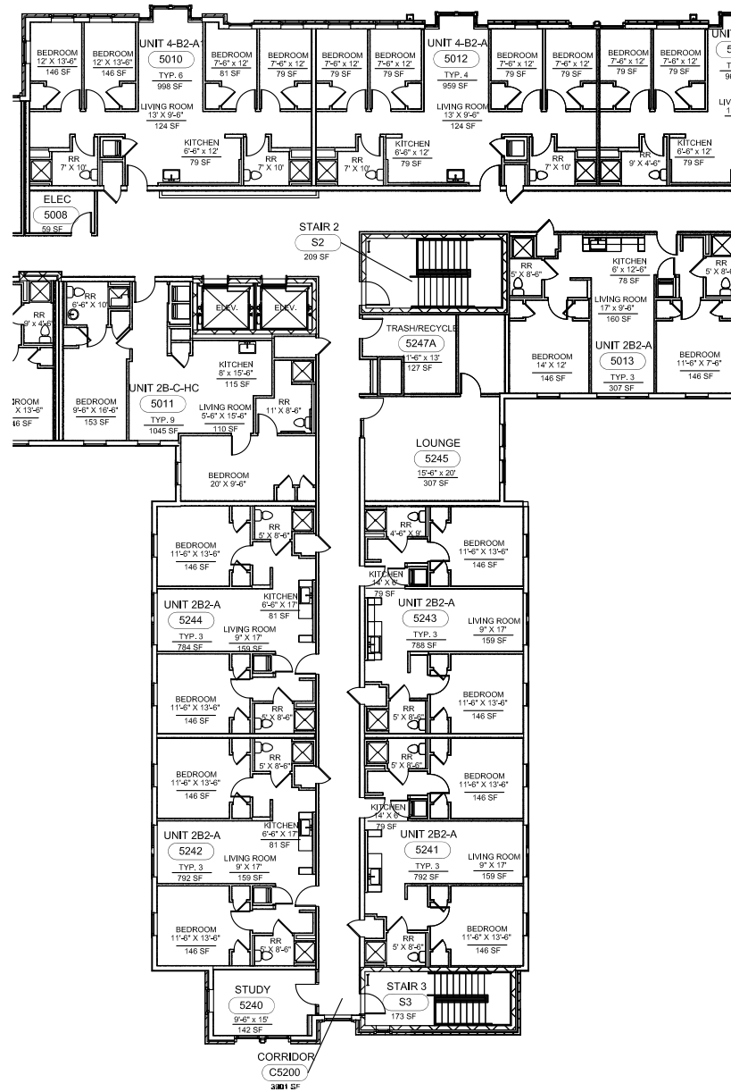
AREA B - FIFTH FLOOR NOT TO SCALE
