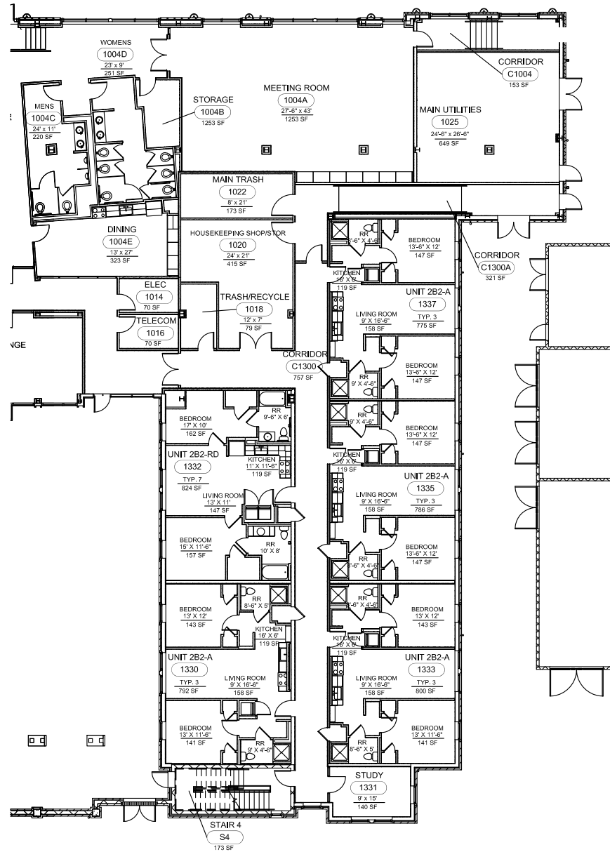
AREA C - FIRST FLOOR NOT TO SCALE
