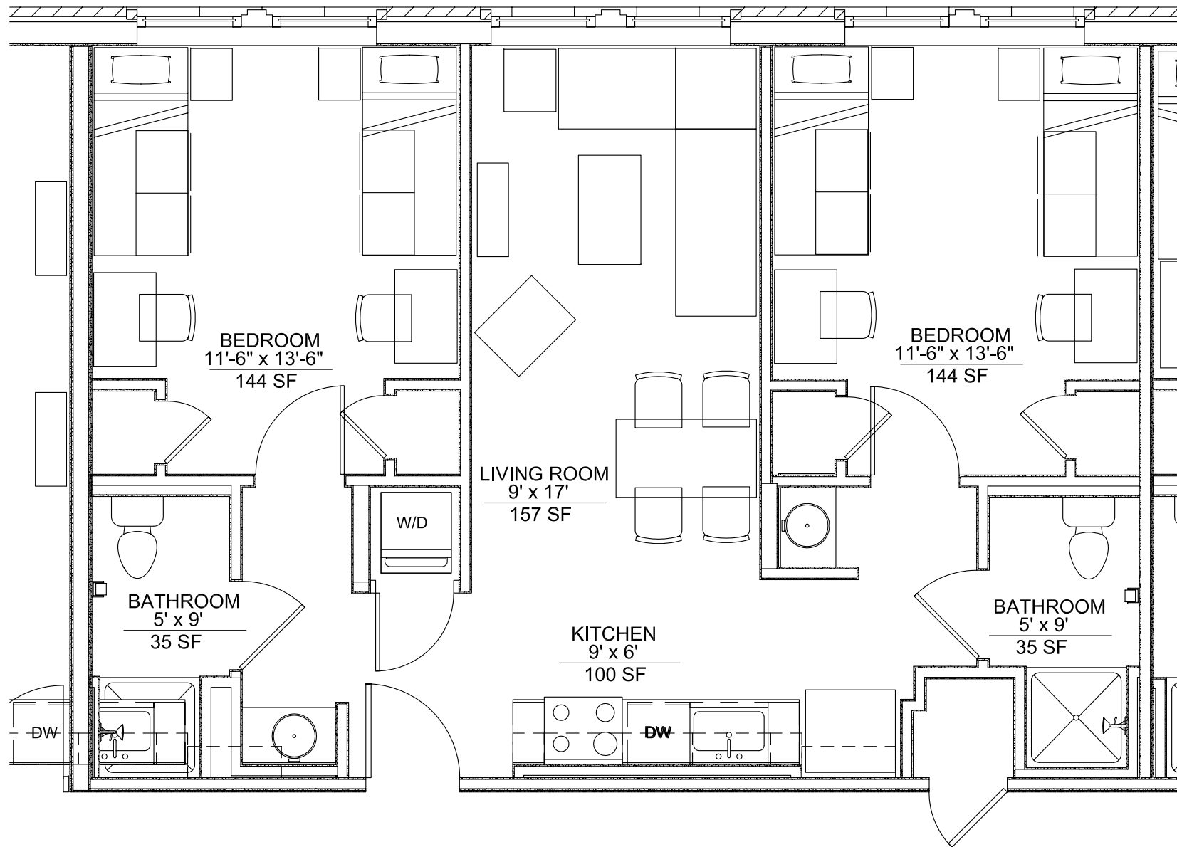
FURNITURE TYPICAL 3 TWO BEDROOM UNIT
