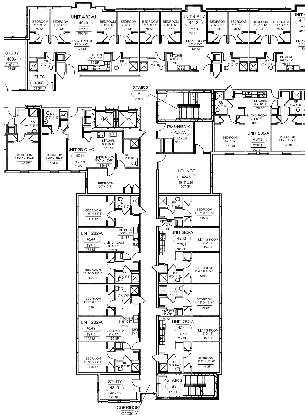
AREA B - FOURTH FLOOR NOT TO SCALE
